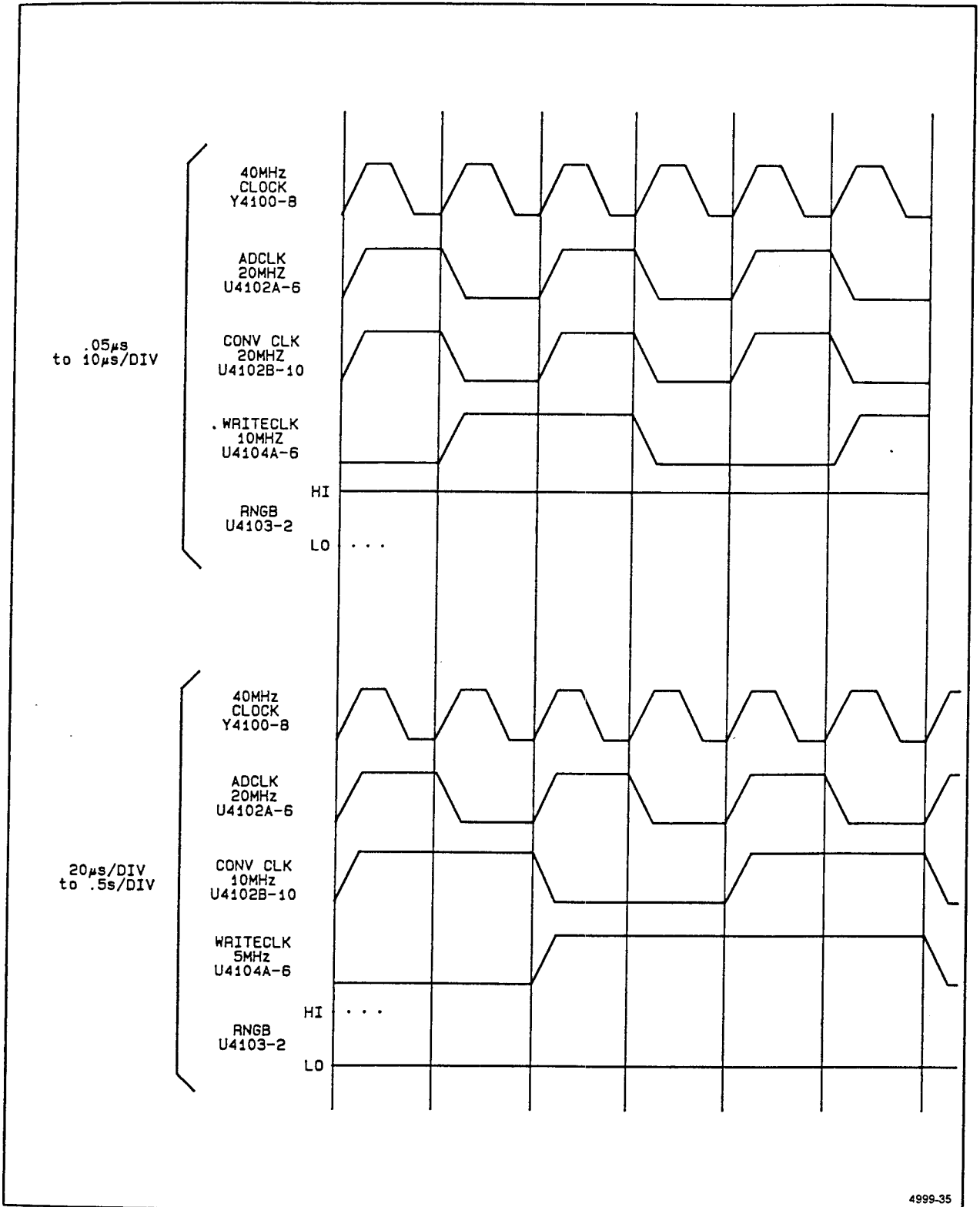
Figure 3-10. Clock timing.
