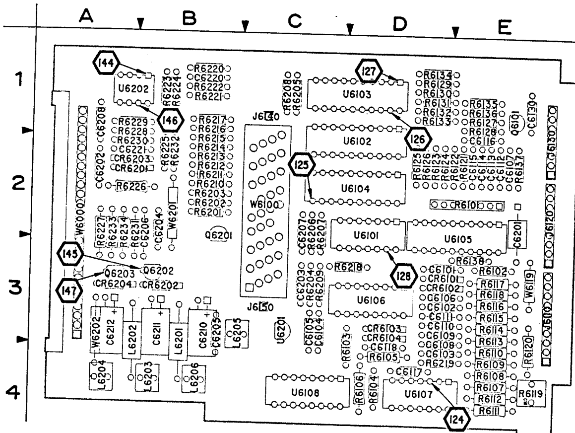
Figure 9-22. A11A1—Input/Output board.
