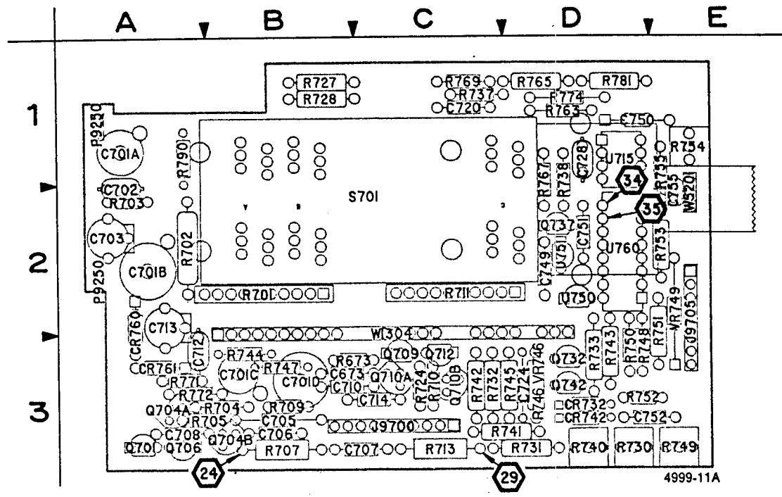
Figure 9-14. A4—Timing board.
