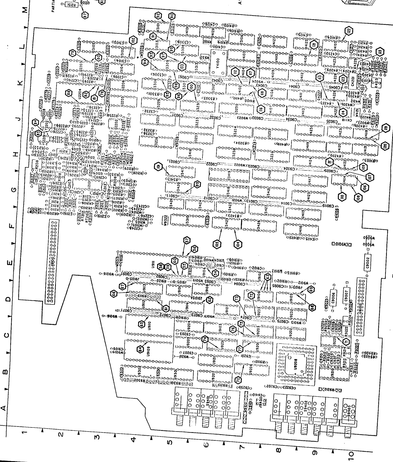
Figure 9-21. A10—Storage board.
