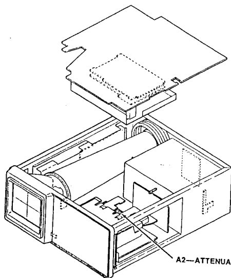
Figure 9-6. A2—Attenuator board.
