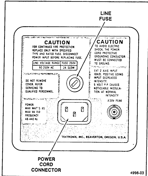
Figure 2-3. Fuse holder and detachable power-cord connector.
